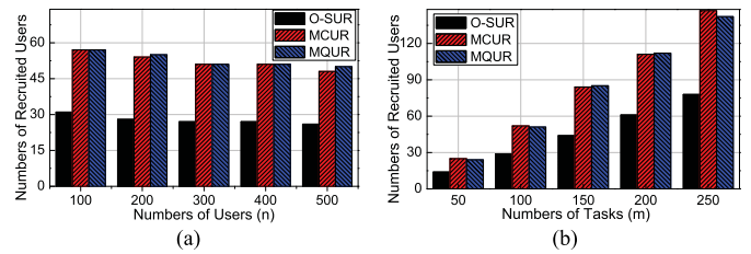
Fig. 3. The performance evaluation of O-SUR. (a) |\Phi| vs. n . (b) |\Phi| vs. m .
