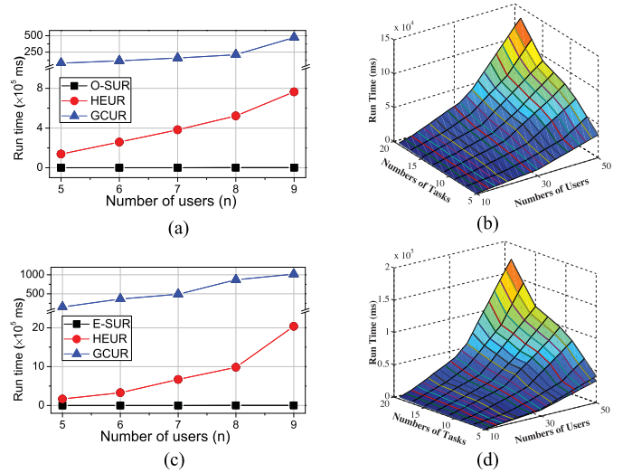
Fig. 8. Performance evaluations: Run time of O-SUR and E-SUR. (a) Comparison for O-SUR. (b) Run time of O-SUR. (c) Comparison for E-SUR. (d) Run time of E-SUR.
