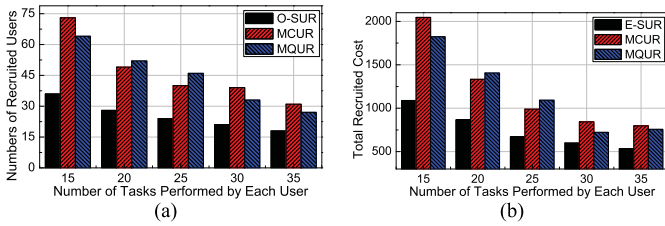
Fig. 7. Evaluation on the parameter \rho . (a) |\Phi| vs. \rho . (b) C(\Phi) vs. \rho .
