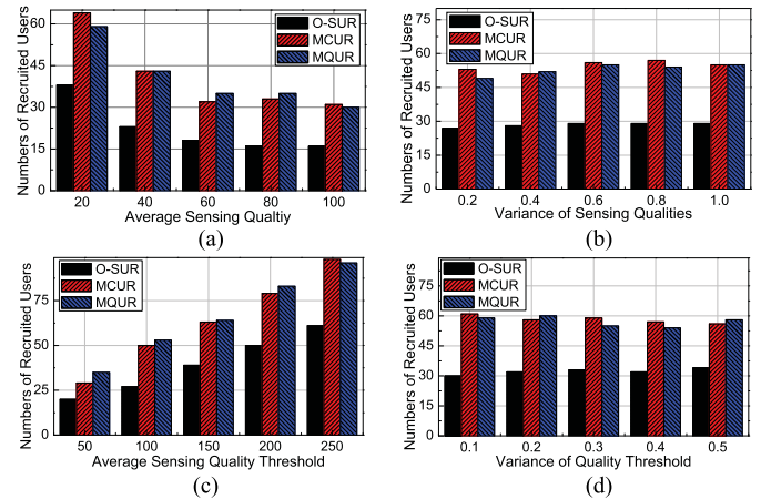
Fig. 4. Performance comparisons of O-SUR: Number of recruited workers versus sensing quality and threshold. (a) |\Phi| vs. \bar{q} . (b) |\Phi| vs. \sigma . (c) |\Phi| vs. \bar{\theta} . (d) |\Phi| vs. \mu .
