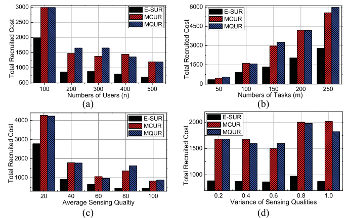
Fig. 5. Performance comparisons of E-SUR: Total recruited cost versus the numbers of tasks and workers and sensing quality. (a) C(\Phi) vs. n . (b) C(\Phi) vs. m . (c) C(\Phi) vs. \bar{q} . (d) C(\Phi) vs. \sigma .
