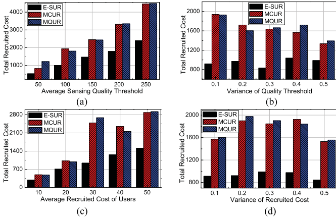
Fig. 6. Performance comparisons of E-SUR: Total recruited cost versus quality threshold and cost. (a) C(\Phi) vs. \bar{\theta} . (b) C(\Phi) vs. \mu . (c) C(\Phi) vs. \bar{c} . (d) C(\Phi) vs. \kappa .
